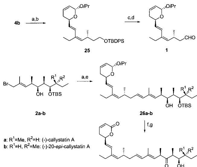
Scheme 7. Synthesis of (–)-callystatin A and its C-20-epimer. a) \text{PBu}_3 , \text{CH}_3\text{CN} , RT. b) 3 , \text{KOtBu} , toluene, 0^\circ\text{C} , 86% over two steps. c) TBAF, THF, RT. d) (\text{COCl})_2 , DMSO, \text{EtN}(\text{iPr})_2 , \text{CH}_2\text{Cl}_2 , -78^\circ\text{C} , 91% over two steps. e) 1 , \text{LiCH}_2\text{S}(\text{O})\text{CH}_3 , toluene, -78^\circ\text{C} , 76% ( 26a ), 73% ( 26b ). f) PCC, \text{AcOH} , 4 Å MS, \text{C}_6\text{H}_6 , RT. g) \text{HF}\cdot\text{pyridine} , THF, RT, 72% (callystatin A), 69% (20- epi -callystatin A). TBAF = tetrabutylammonium fluoride, PCC = pyridinium chlorochromate.
