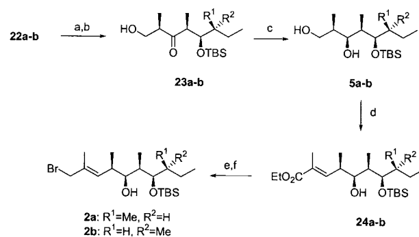
Scheme 6. Synthesis of allylic bromides 2a–b . a) TBSOTf, 2,6-lutidine, CH 2 Cl 2 , RT, 98 % ( 22a ), 99 % ( 22b ). b) H 2 , Pd/C, EtOH, RT, 95 % ( 23a ), 98 % ( 23b ). c) DIBAL-H, CH 2 Cl 2 , –78 °C, 87 % ( 5a ), 86 % ( 5b ). d) 1) (COCl) 2 , DMSO, EtN( i Pr) 2 , CH 2 Cl 2 , –78 °C; 2) Ph 3 P=C(CH 3 )CO 2 Et, CH 2 Cl 2 , reflux, 79 % ( 24a ), 52 % ( 24b ). e) DIBAL-H, CH 2 Cl 2 , –78 °C. f) CBr 4 , PPh 3 , 2,6-lutidine, CH 3 CN, RT, 76 % ( 2a ), 81 % ( 2b ) over two steps.
