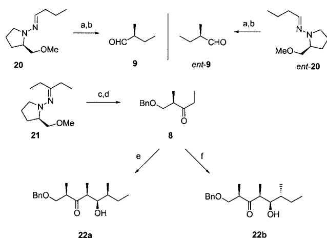
Scheme 5. Diastereoselective aldol coupling between 8 and 9 . a) 1) LDA, THF, 0 °C; 2) MeI, –100 °C. b) O 3 , CH 2 Cl 2 , –78 °C, 72 % ( 9 ), 67 % ( ent-9 ) over two steps. c) 1) LDA, Et 2 O, 0 °C; 2) BOMCl, –100 °C. d) O 3 , CH 2 Cl 2 , –78 °C, 79 % over two steps. e) 1) Sn(OTf) 2 , Et 3 N, CH 2 Cl 2 , –78 °C; 2) 9 , –78 °C, 87 % (97 % ds ). f) 1) TiCl 4 , EtN( i Pr) 2 , CH 2 Cl 2 , –78 °C; 2) ent-9 , –78 °C, 96 % (94 % ds ).
