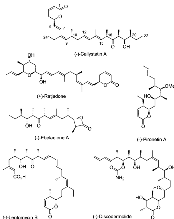
Figure 1. (–)-Callystatin A and other structurally related natural products.
