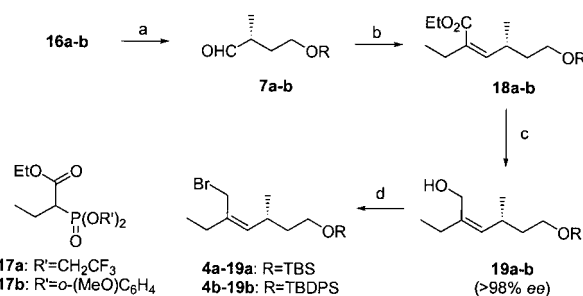
Scheme 4. Synthesis of the allylic bromides 4a–b . a) \text{O}_3 , \text{CH}_2\text{Cl}_2 , -78^\circ\text{C} , 86 % ( 7a ), 77 % ( 7b ). b) 17b , NaH, THF, 0^\circ\text{C} , 85 % ( 18a ), 91 % ( 18b ). c) DIBAL-H, \text{CH}_2\text{Cl}_2 , -78^\circ\text{C} , 95 % ( 19a ), 96 % ( 19b ). d) \text{CBr}_4 , \text{PPh}_3 , \text{CH}_3\text{CN} , RT, 5 % ( 4a , R = TBS), 95 % ( 4b , R = TBDPS).
