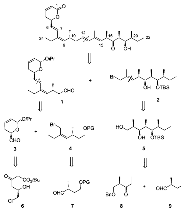
Scheme 1. Retrosynthetic analysis for (–)-callistatin A.
