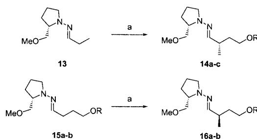
Scheme 3. Synthesis of the \alpha -alkylated hydrazones 14a–c and 16a–b . a) see Table 1.
