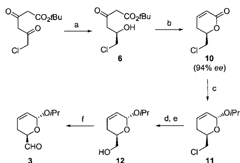
Scheme 2. Synthesis of the aldehyde 3 . a) dried baker's yeast, XAD-7/ \text{H}_2\text{O} , RT, 50 %. b) 1) \text{NaBH}_4 , \text{EtOH} , 0^\circ\text{C} ; 2) p\text{TsOH} (cat), toluene, 120^\circ\text{C} , 78 %. c) 1) DIBAL-H, \text{CH}_2\text{Cl}_2 , -78^\circ\text{C} ; 2) i\text{PrOH} , PPTS, benzene, 80^\circ\text{C} , 79 %. d) TBAA, NMP, 85^\circ\text{C} , 89 %. e) \text{K}_2\text{CO}_3 , MeOH, 97 %. f) (\text{COCl})_2 , DMSO, \text{EtN}(i\text{Pr})_2 , \text{CH}_2\text{Cl}_2 , -78^\circ\text{C} , 95 %. TBAA = tetrabutylammonium acetate, NMP = N -methyl-2-pyrrolidinone.
